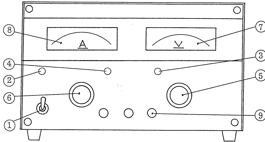
Fig. 3-1 Front Panel
