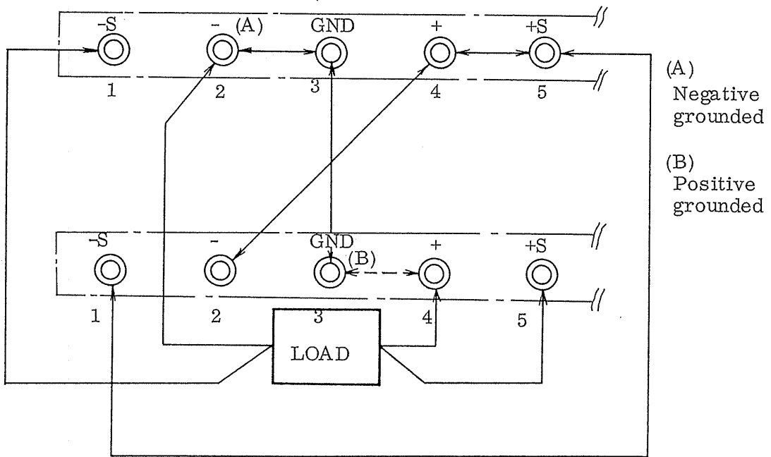
Fig. 3-6 Sampling terminal connection diagram in series connection
