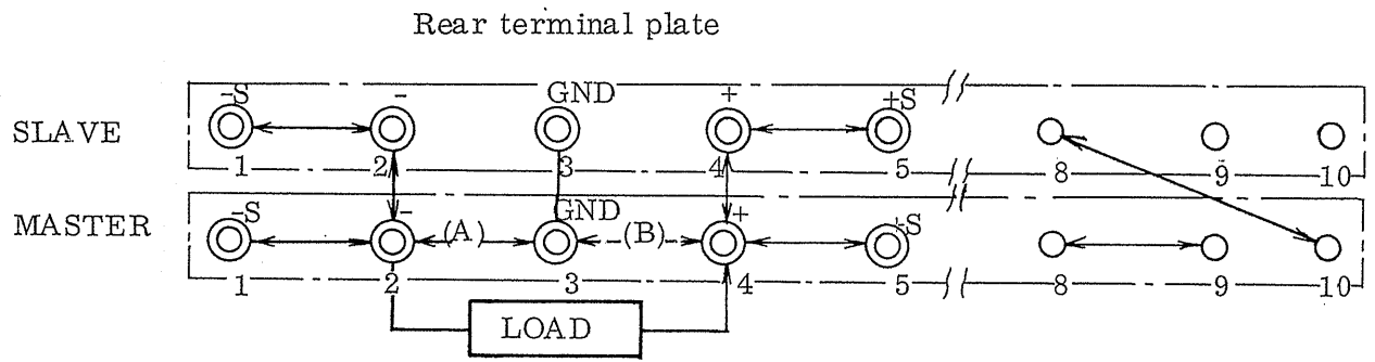
Fig. 3-10 One-control parallel operation master, slave, load
