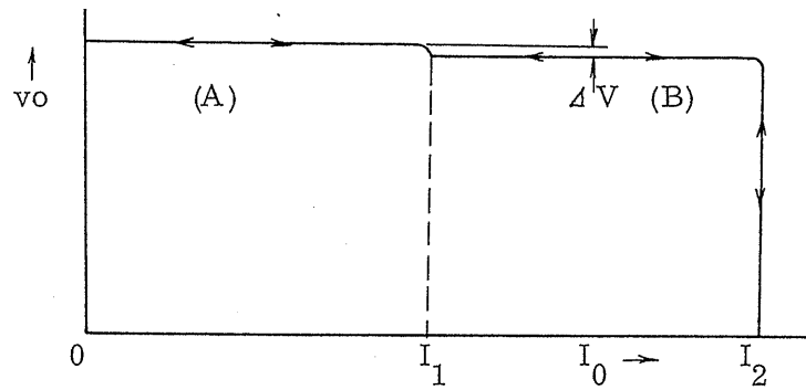
Fig. 3-9 Characteristics diagram
